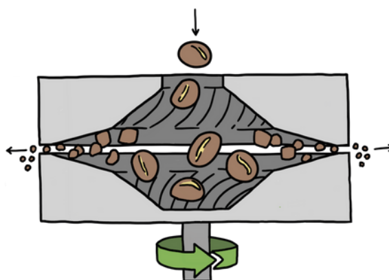
FLAT BURR
